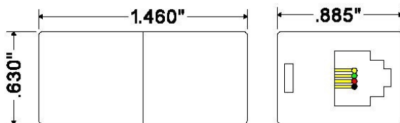
FIGURE 2 FEMALE TO FEMALE CABLE ADAPTOR STRAIGHT THROUGH P/N E-04.10.8
